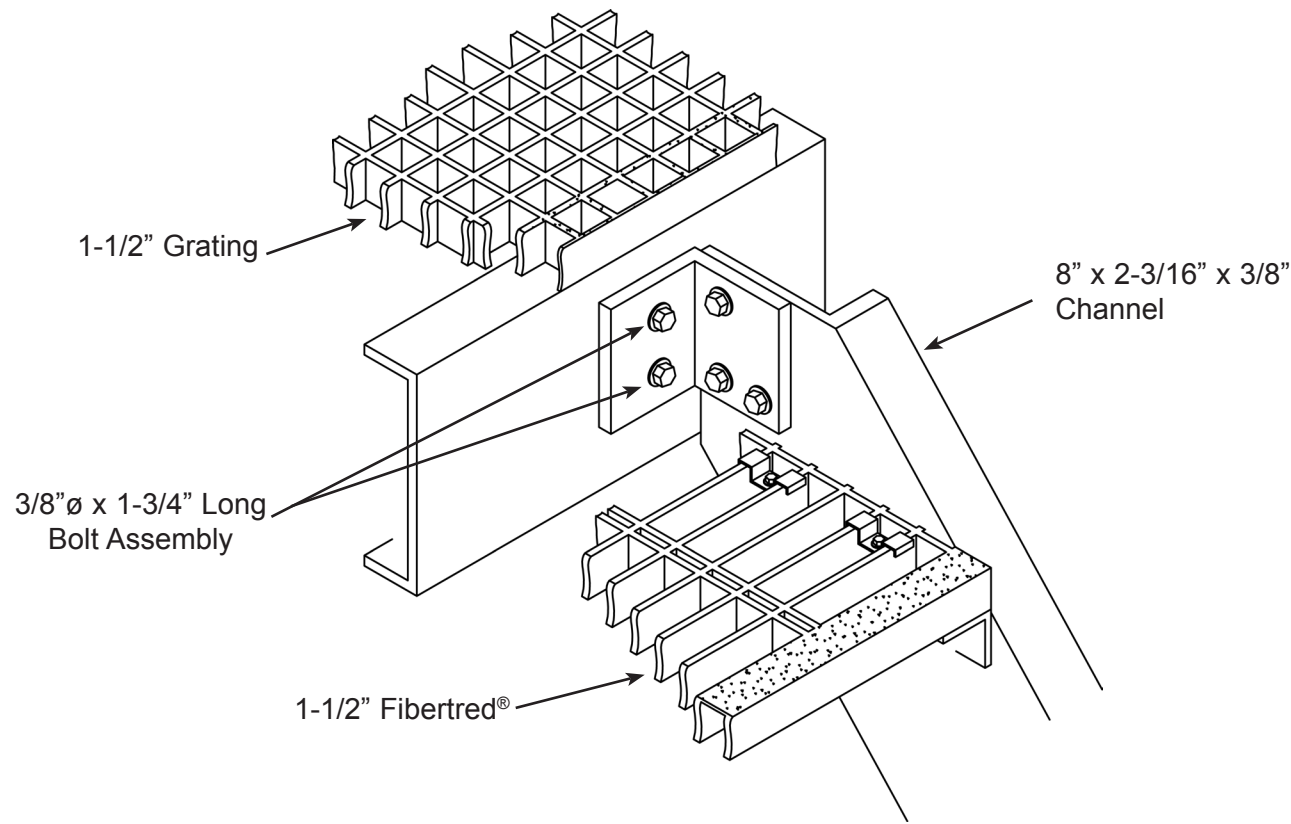
DRAWING U: TOP STAIR STRINGER MOUNT
