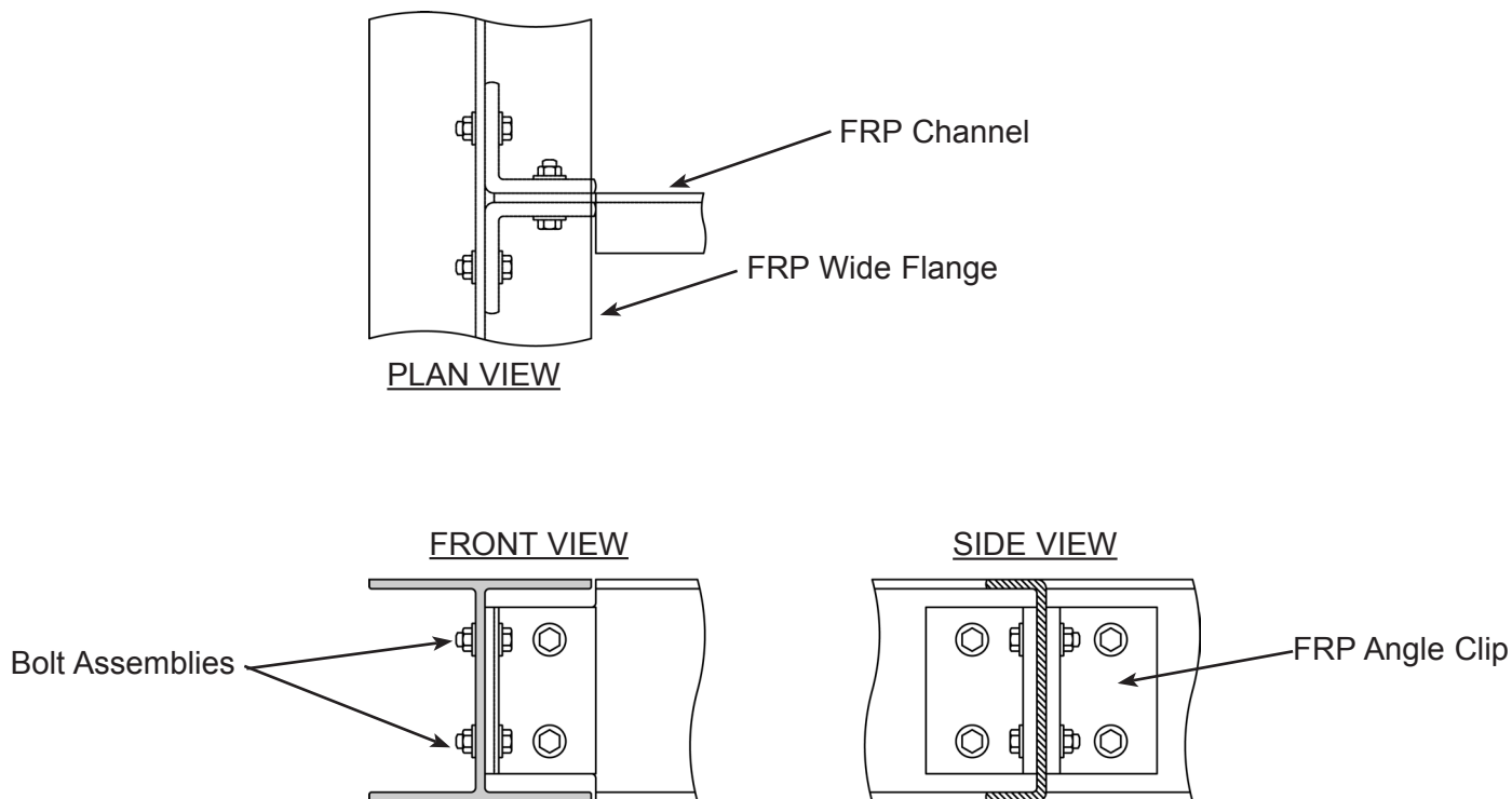
DRAWING R: WIDE FLANGE TO CHANNEL CONNECTION
